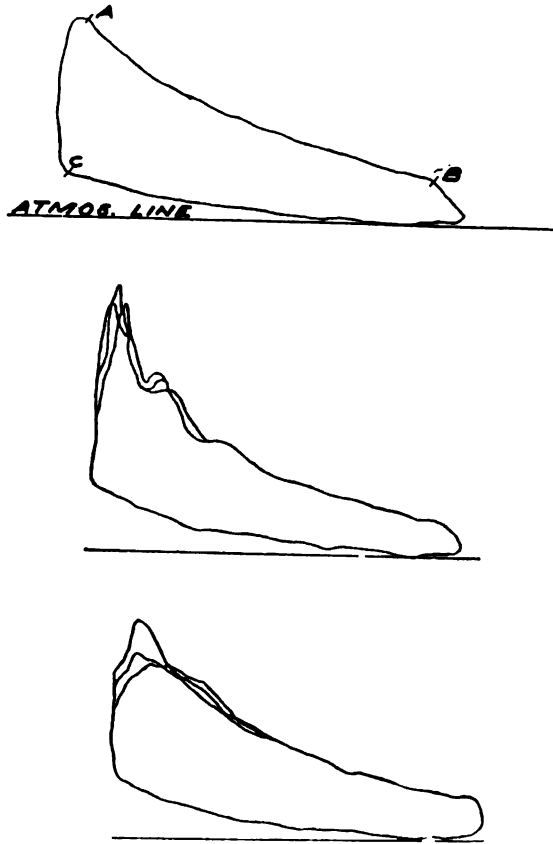
FIG. 300.—Gas Engine Indicator Cards. The first diagram is an average good card, showing, however, some slight fluctuations in the lines. The explosion line is from C to A; the expansion, from A to B; the exhaust at B. The suction stroke generally approximates the atmospheric line, from which the curve of compression rises to C. The second diagram is from an engine running under half load; the third from one at full load. Both exhibit the variations in the expansion curve, usually attributed to consecutive explosions. The second and third cards are composites of three successive strokes each.
